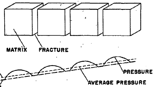
FIG. 2 — SCHEMATIC REPRESENTATION OF THE PRESSURE DISTRIBUTION IN THE MODEL.
