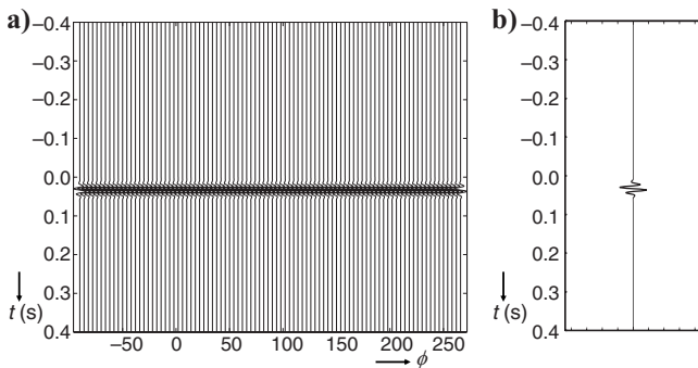
Figure 8. (a) The integrand of \mathcal{L}(G_A, G_B) . (b) The sum of all traces in (a).
