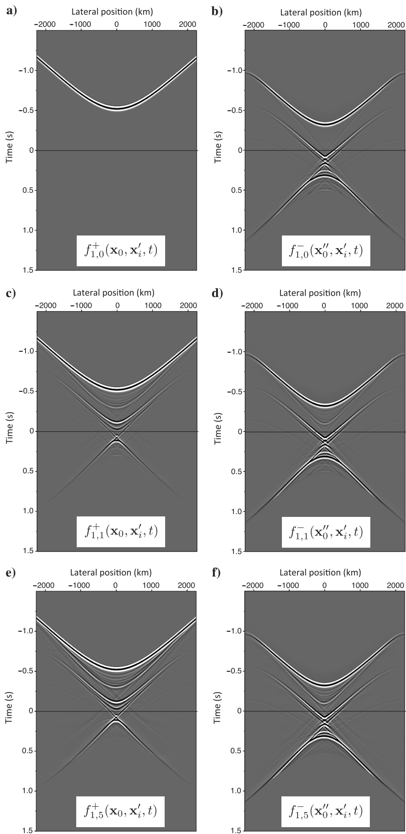
Figure 6. The focusing functions f_{1,k}^+(\mathbf{x}_0, \mathbf{x}'_i, t) and f_{1,k}^-(\mathbf{x}'_0, \mathbf{x}'_i, t) , for fixed \mathbf{x}'_i and variable \mathbf{x}_0 and \mathbf{x}'_0 , for k = 0 (Figure 6a and 6b), k = 1 (Figure 6c and 6d), and k = 5 (Figure 6e and 6f).
