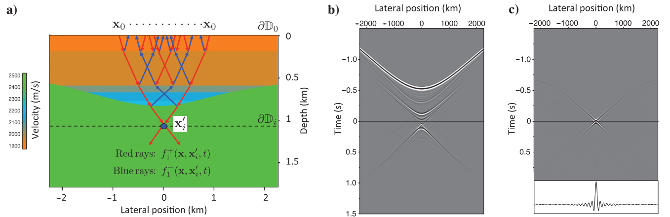
Figure 4. Illustration of the actual focusing function f_1^+(\mathbf{x}, \mathbf{x}_i', t) . (a) Ray diagram of the actual focusing function. (b) Actual focusing function at \partial\mathbb{D}_0 . (c) Its response at \partial\mathbb{D}_i . Inset: cross section of the focus at the central frequency.
