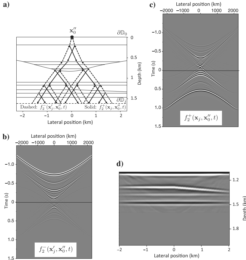
Figure 15. (a) Ray diagram of the focusing functions f_{2,0}^-(\mathbf{x}'_j, \mathbf{x}''_0, t) and f_{2,0}^+(\mathbf{x}_j, \mathbf{x}''_0, t) . (b) The retrieved focusing function f_{2,0}^-(\mathbf{x}'_j, \mathbf{x}''_0, t) , for fixed \mathbf{x}''_0 and variable \mathbf{x}'_j . (c) The retrieved focusing function f_{2,0}^+(\mathbf{x}_j, \mathbf{x}''_0, t) , for fixed \mathbf{x}''_0 and variable \mathbf{x}_j . (d) Marchenko image of the target area above \partial\mathbb{D}_j , obtained by resolving R^\cap(\mathbf{x}_j, \mathbf{x}'_j, t) from the focusing functions, followed by standard imaging.
