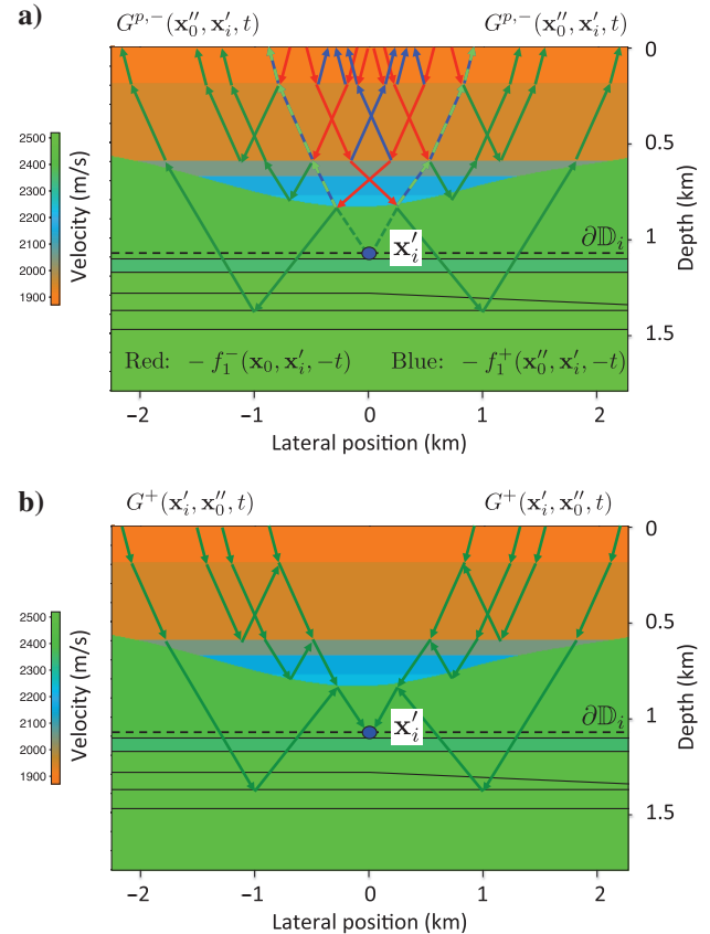
Figure 12. Physical interpretation of equation 35. (a) The incident field -f_1^-(\mathbf{x}_0, \mathbf{x}'_i, -t) (red rays) gives rise to -f_1^+(\mathbf{x}_0'', \mathbf{x}'_i, -t) (blue rays) and the Green's function G^{p,-}(\mathbf{x}_0'', \mathbf{x}'_i, t) (green rays). (b) After subtracting -f_1^+(\mathbf{x}_0'', \mathbf{x}'_i, -t) and applying source-receiver reciprocity, the Green's function G^+(\mathbf{x}'_i, \mathbf{x}_0'', t) remains.
