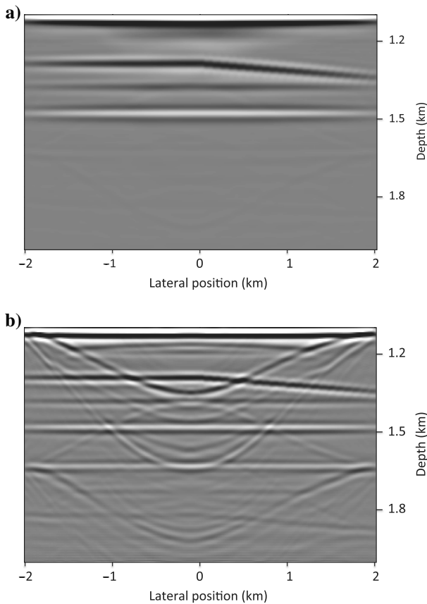
Figure 14. (a) Marchenko image of the target zone, obtained from the redatumed response R^\cup(\mathbf{x}_i, \mathbf{x}_i', t) . Note that this image has been obtained without first resolving the reflection properties of the overburden. (b) Standard image, obtained from the reflection response R^\cup(\mathbf{x}_0'', \mathbf{x}_0, t) at the surface.
