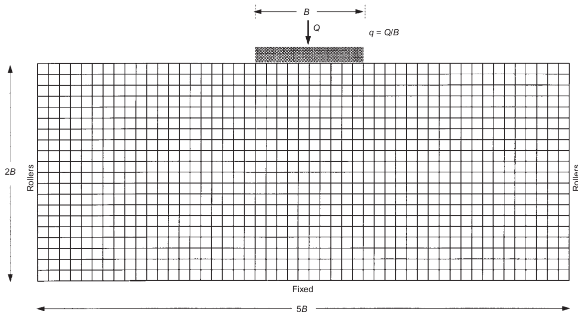
Fig. 2. Mesh used in probabilistic bearing capacity analyses
