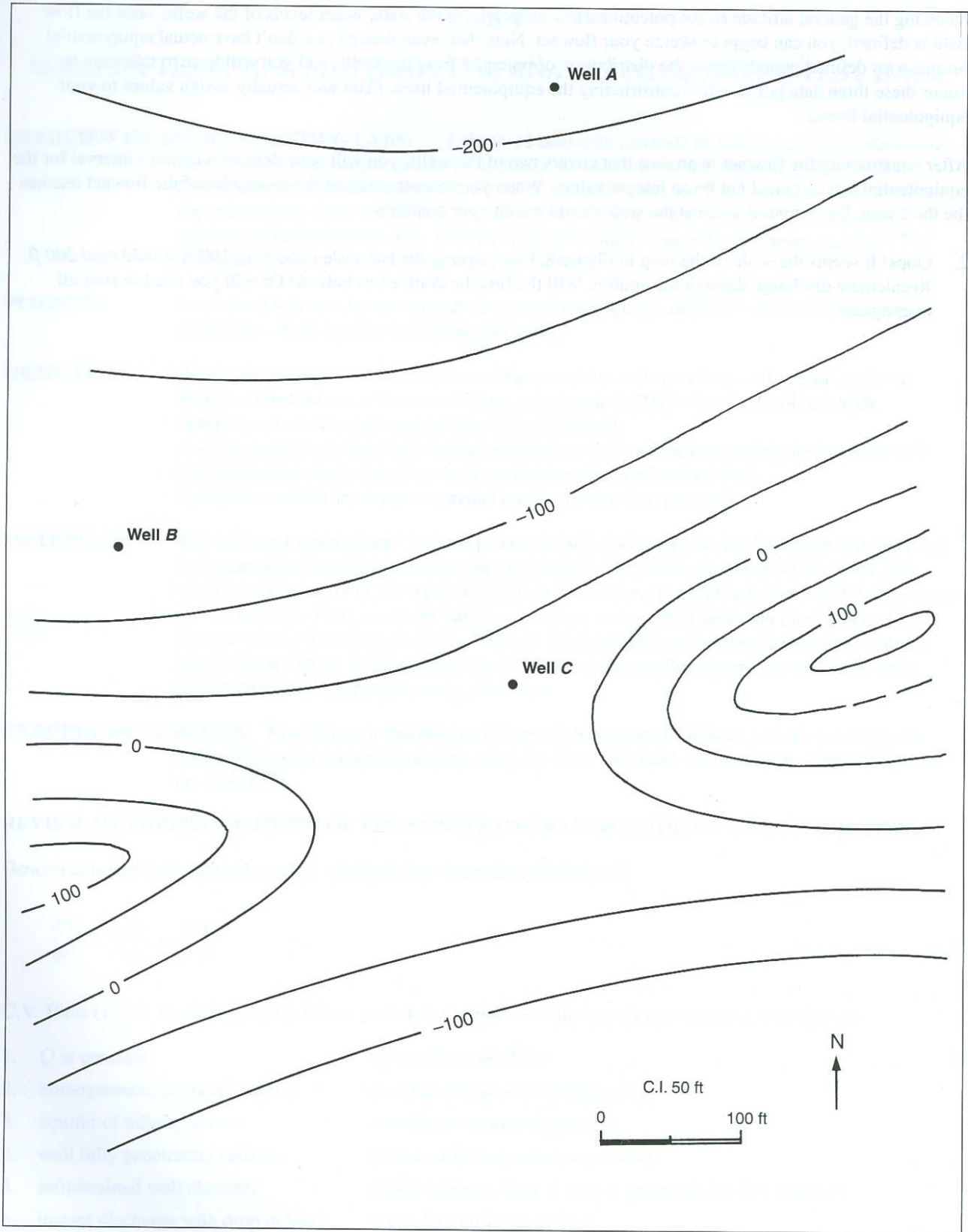
Figure 8.3—Structure contour map of the top of Precambrian granite (contour interval 50 feet).
