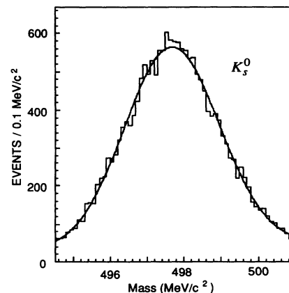
FIG. 1. Invariant mass for the exclusive K_S^0 events fit to a Gaussian and a linear background shown explicitly. The standard deviation is 1.28 MeV/c 2 .
