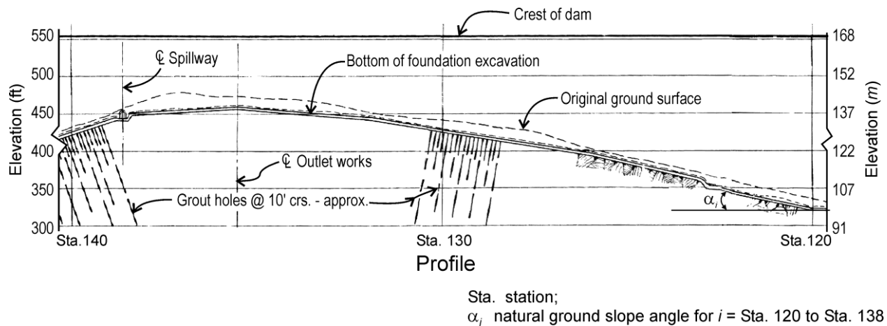
Figure 2. Profile view along the centerline of the San Luis Dam site between stations 120 and 140.
