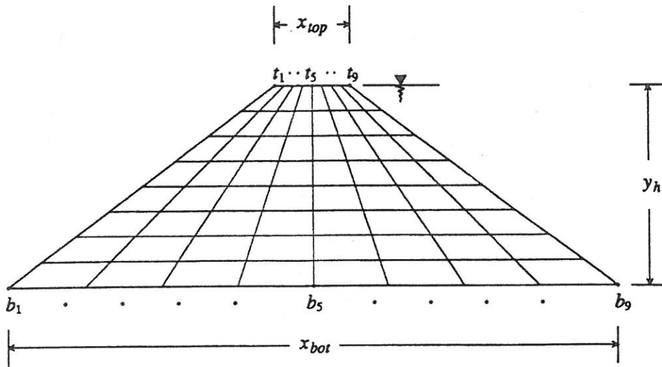
Figure 3. Earth dam dimensions illustrating top and bottom nodal x -co-ordinate labeling
