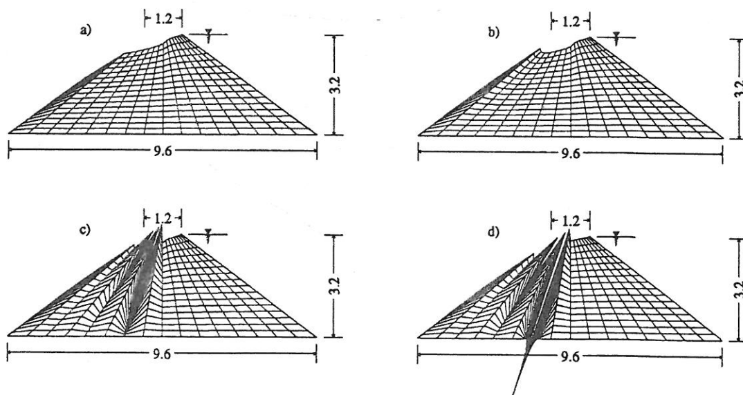
Figure 2. Divergent iteration sequence (a)–(d) due to excessive element distortion
