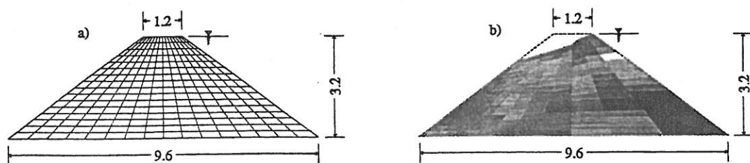
Figure 1. Finite element mesh of earth dam (a) with example realization of permeability field and free surface (b)
