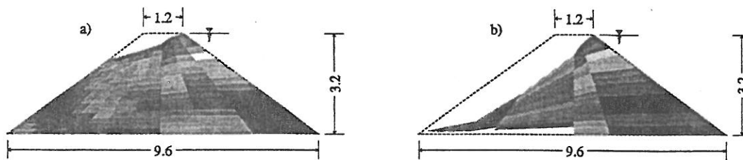
Figure 4. Converged free surface results obtained using geometric spacing for undrained, (a), and drained, (b), earth dams
