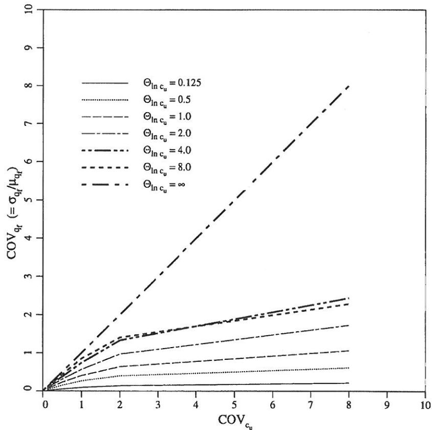
Fig. 7. Estimated coefficient of variation of bearing capacity ( COV_{q_r} ) as function of undrained shear strength statistics \Theta_{\ln c_u} and COV_{c_u}
