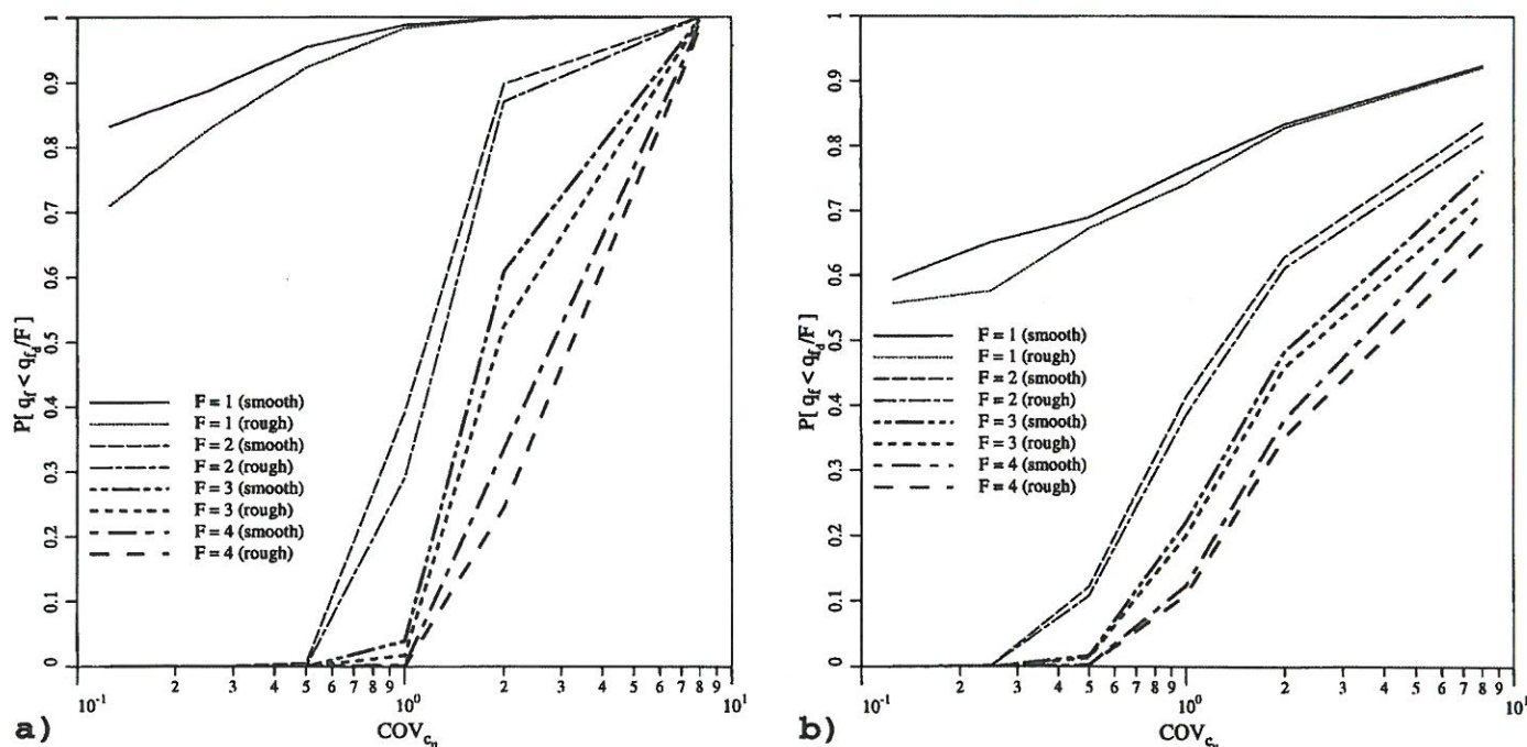
Fig. 16. Comparison of probability of design failure for smooth and rough footings: \Theta_{ln c_w} = (a) 0.5, (b) 8
