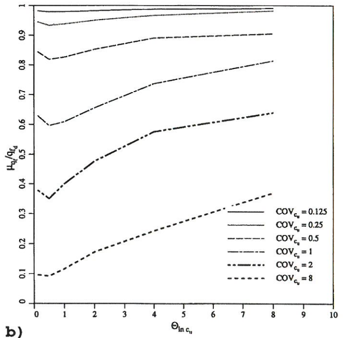
Fig. 6. Estimated mean bearing capacity as function of undrained shear strength statistics \Theta_{\ln c_u} and COV_{c_u}
