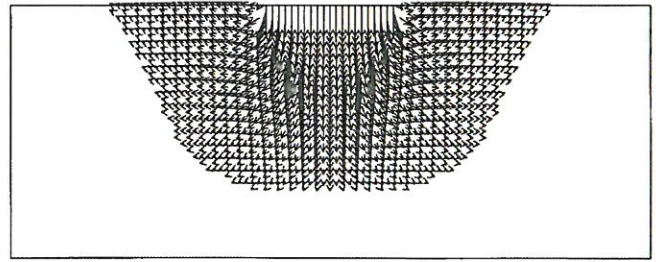
Fig. 3. Displacement vector at failure of rough footing in deterministic analysis
