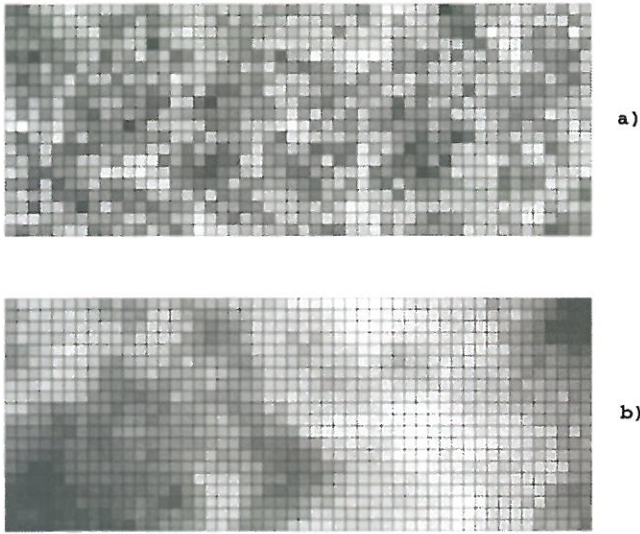
Fig. 5. Influence of \Theta_{\ln c_u} on random field generation ( COV_{c_u} = 1 ): \Theta_{\ln c_u} = (a) 0.125, (b) 8
