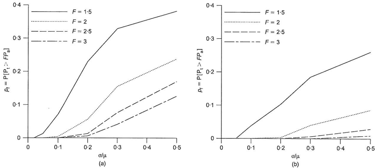
Fig. 3. Estimated probability that actual load exceeds design load, \hat{p}_r , for \theta/H = 1 : (a) \phi' and \gamma fields are independent ( \rho = 0 ); (b) the two fields are strongly correlated ( \rho = 0.8 )
