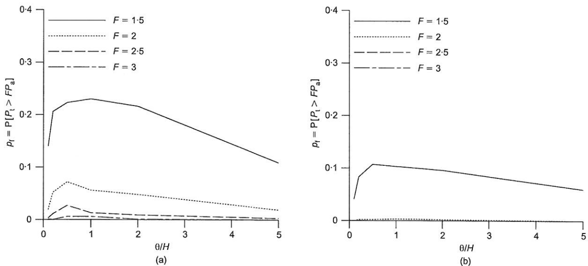
Fig. 4. Estimated probability that actual load exceeds design load, \hat{p}_r , for \sigma/\mu = 0.2 : (a) \phi' and \gamma fields are independent ( \rho = 0 ); (b) the two fields are strongly correlated ( \rho = 0.8 )
