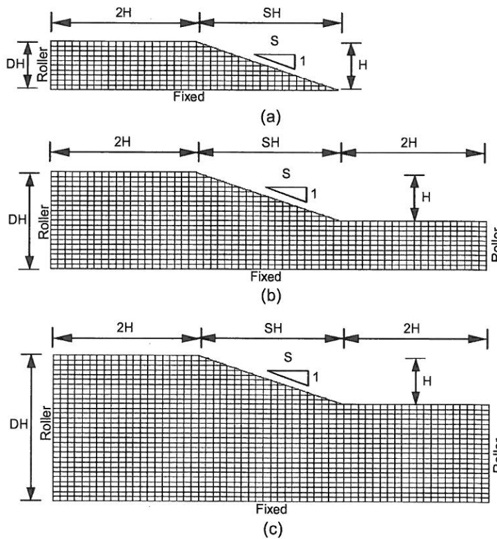
Figure 2: Meshes used for RFEM slope stability analyses with slope S and D = (a) 1; (b) 2; (c) 3.
