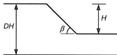
Figure 1: Geometry of cohesive slope problem.
