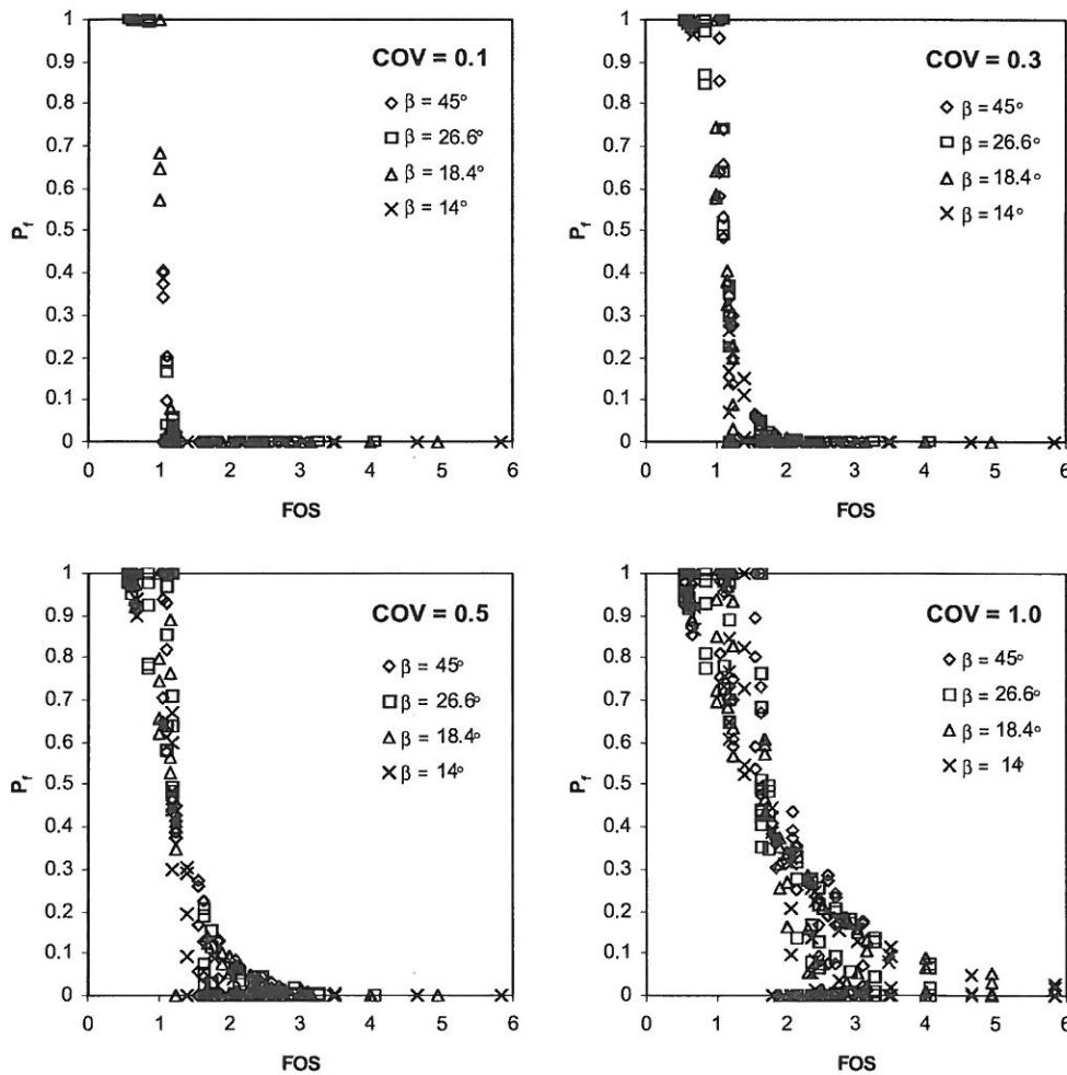
Figure 4: P_f versus FOS for COV = 0.1, 0.3, 0.5, and 1.0 .
