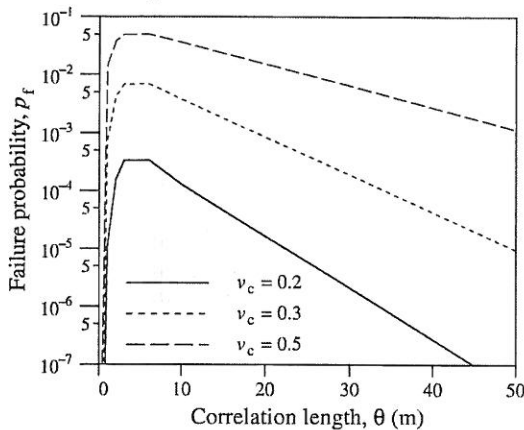
Fig. 2. Failure probability versus correlation length for \Psi_u = 1.15 (low consequence), \phi_{gu} = 0.50 , and r = 4.5 m.
