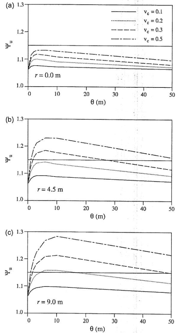
Fig. 6. Consequence factor versus correlation length for various sampling locations at low consequence level ( p_m = 1/1000 ) using best estimates of \varphi_{gu} from Fig. 3: (a) r = 0.0 m; (b) r = 4.5 m; (c) r = 9.0 m.
