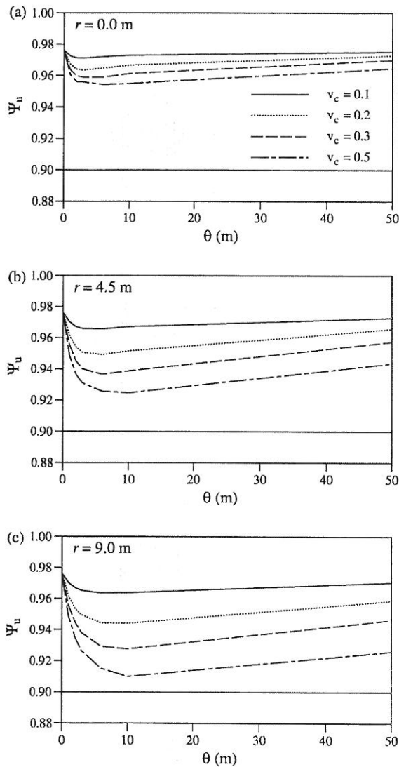
Fig. 5. Consequence factor versus correlation length for various sampling locations at high consequence level ( p_m = 1/10\,000 ) using best estimates of \varphi_{gu} from Fig. 3: (a) r = 0.0 m; (b) r = 4.5 m; (c) r = 9.0 m.
