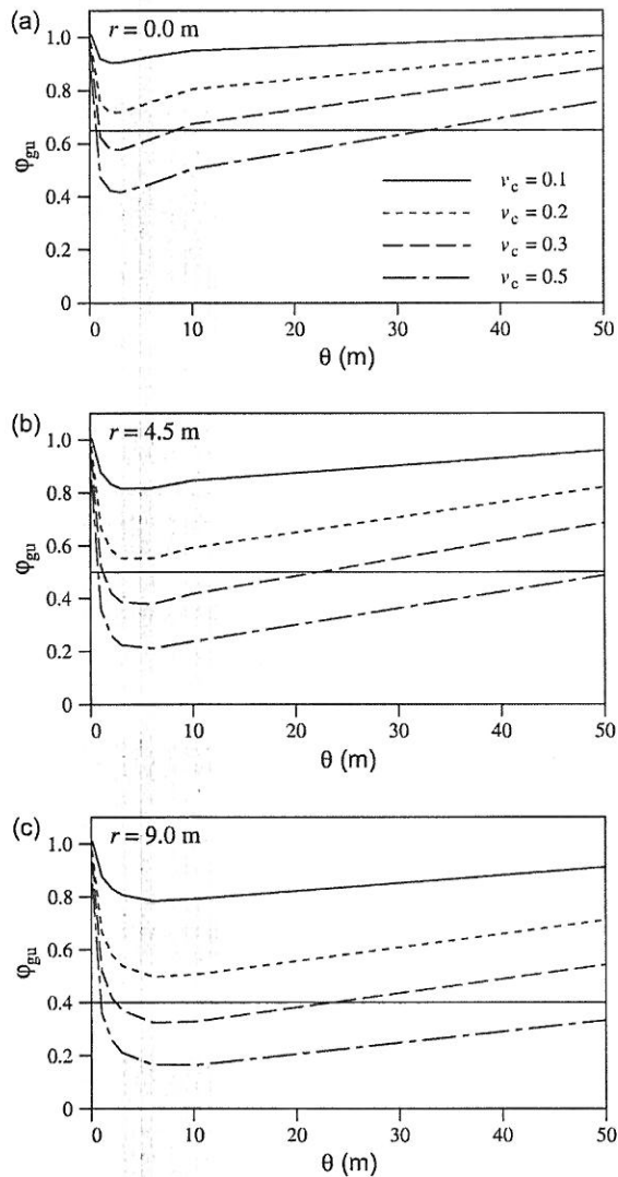
Fig. 3. Resistance factors versus correlation length for medium consequence level ( \Psi_u = 1.0 ) at the three site understanding levels: (a) high ( r = 0 m), (b) medium ( r = 4.5 m), and (c) low ( r = 9 m). Solid horizontal lines show selected design resistance factor values for each site understanding level.
