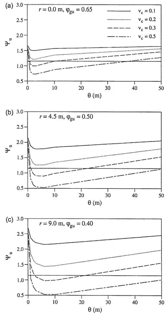
Fig. 8. Consequence factor versus correlation length for various sampling locations at low consequence level ( p_m = 1/1000 ) using proposed design values of \phi_{gu} : (a) r = 0.0 m, \phi_{gu} = 0.65 ; (b) r = 4.5 m, \phi_{gu} = 0.50 ; (c) r = 9.0 m, \phi_{gu} = 0.40 .
