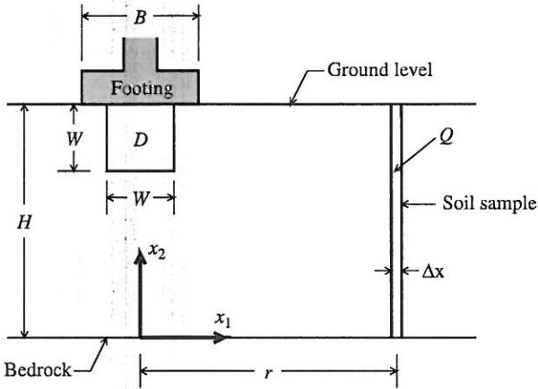
Fig. 1. Averaging regions used to predict probability of bearing capacity failure.
