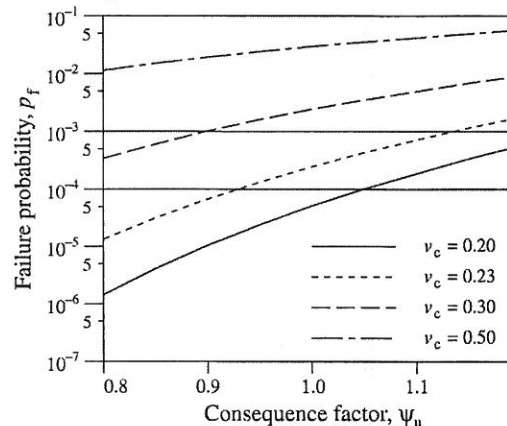
Fig. 4. Failure probability versus consequence factor for \theta = 6 m, r = 4.5 m, and \phi_{gu} = 0.50 .
