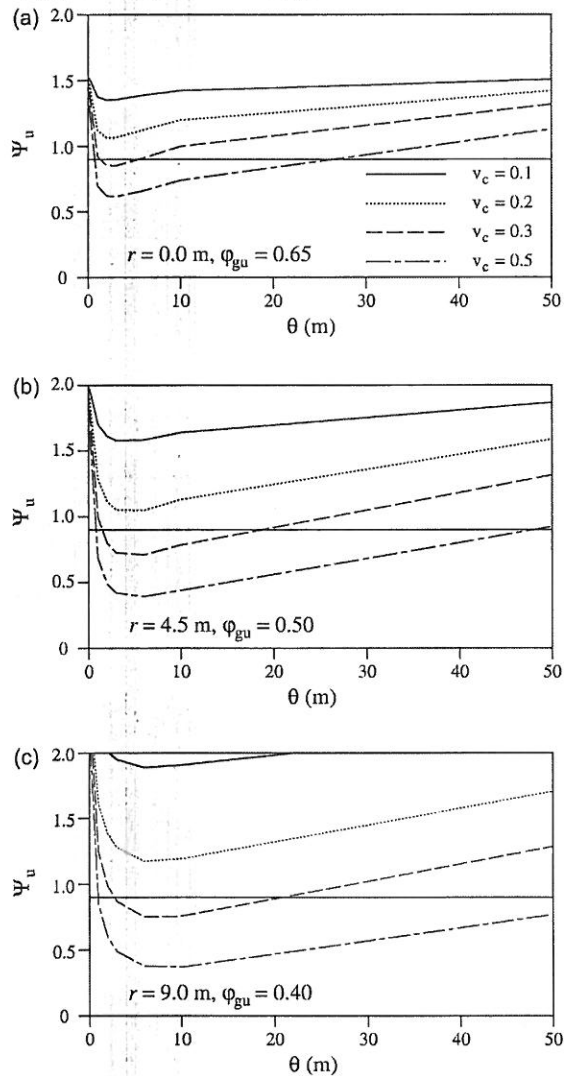
Fig. 7. Consequence factor versus correlation length for various sampling locations at high consequence level ( p_m = 1/10\,000 ) using proposed design values of \phi_{gu} : (a) r = 0.0 m, \phi_{gu} = 0.65 ; (b) r = 4.5 m, \phi_{gu} = 0.50 ; (c) r = 9.0 m, \phi_{gu} = 0.40 .
