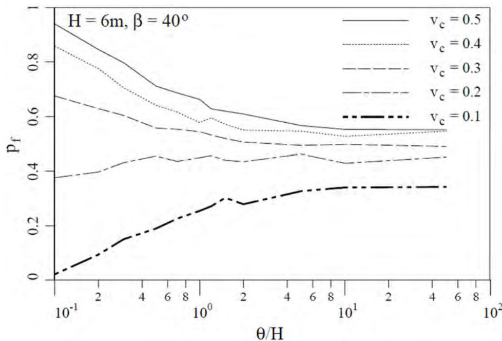
Figure 2. Slope failure probability versus \theta_{\ln c_u} / H for a slope having height H = 6 m, \beta = 40^\circ and various cohesion coefficients of variation, v_c .
