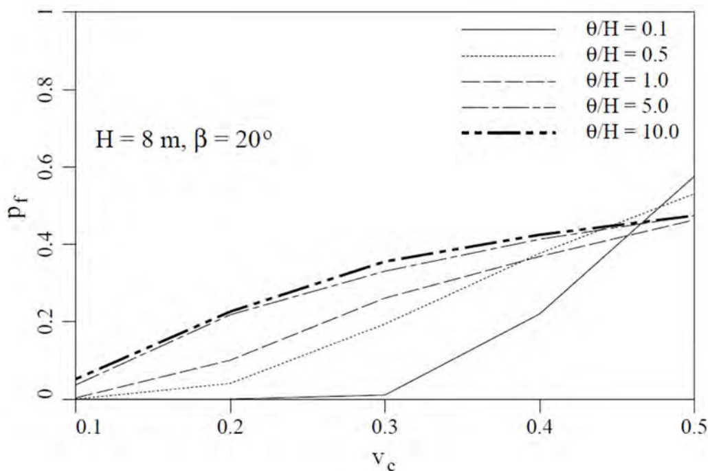
Figure 6. Slope failure probability versus cohesion coefficient of variation, v_c for a slope having height H = 8 m and angle \beta = 20^\circ .
