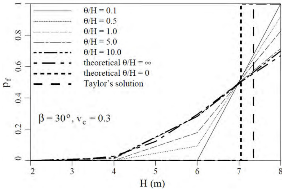
Figure 4. Slope failure probability versus slope height, H for a slope having angle \beta = 30^\circ and coefficient of variation of v_c = 0.3 .
