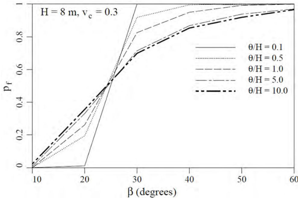
Figure 5. Slope failure probability versus slope angle, \beta for a slope having height H = 8 m and coefficient of variation of v_c = 0.3 .
