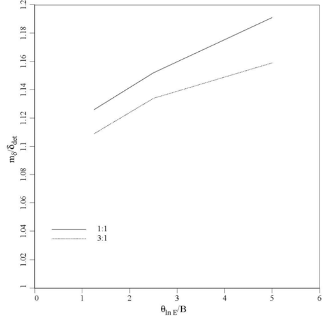
Figure 3. Normalised results for square and 3:1 rectangular footings for CV_E = 0.5 . Mean settlement vs. correlation length
