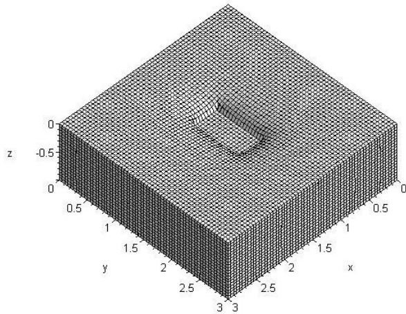
Figure 1, Mesh used for footing settlement study
