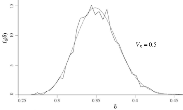
Figure 2. Histogram of RFEM settlement for a 3:1 rectangular footing. Lognormal fit to data is also shown
