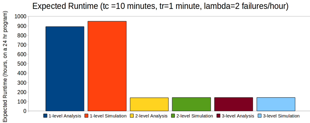
Fig. 11. Comparison of analysis and simulation expected runtimes for the 1-level, 2-level, and 3-level schemes with t_c=10 min, t_r=1 min, and \lambda=2 failures/hour.
