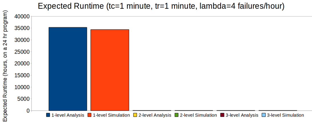
Fig. 8. Comparison of analysis and simulation expected runtimes for the 1-level, 2-level, and 3-level schemes with tc=1 min, tr=1 min, and \lambda=4 failures/hour.
