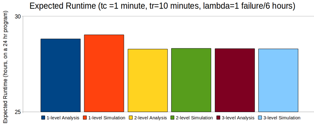
Fig. 7. Comparison of analysis and simulation expected runtimes for the 1-level, 2-level, and 3-level schemes with tc=1 min, tr=10 min, and \lambda=1 failure/6 hours.
