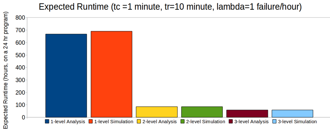
Fig. 9. Comparison of analysis and simulation expected runtimes for the 1-level, 2-level, and 3-level schemes with tc=1 min, tr=10 min, and \lambda=1 failure/hour.
