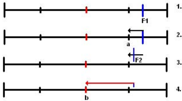
Fig. 2. Flow of a two-failure recovery. 1) Failure occurs at time F1. 2) System attempts to recover to most recent one failure checkpoint (a). 3) Failure occurs while attempting recovery at F2. 4) System recovers to most recent two-failure checkpoint (b).
