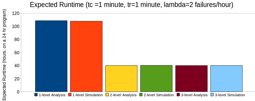
Fig. 10. Comparison of analysis and simulation expected runtimes for the 1-level, 2-level, and 3-level schemes with t_c=1 min, t_r=1 min, and \lambda=2 failures/hour.
