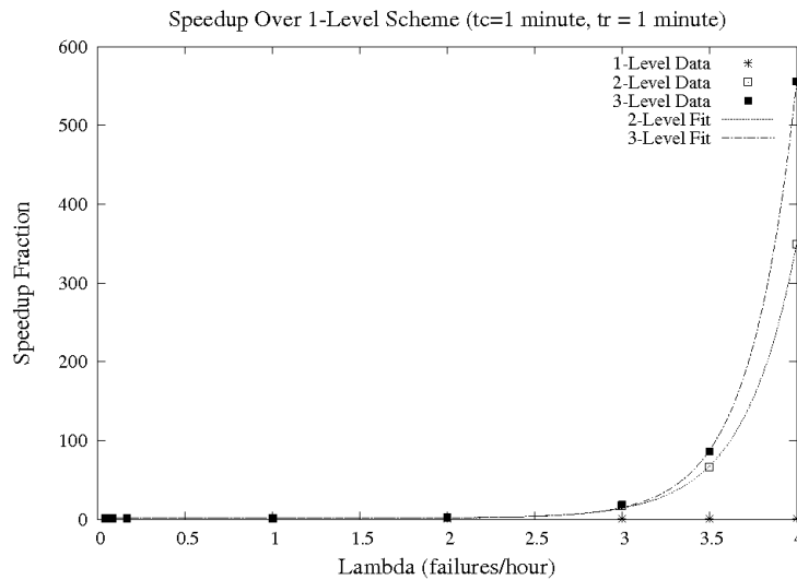
Fig. 14. Speedup fraction of 2-Level and 3-Level schemes over the 1-Level scheme with increasing \lambda . The t_c and t_r parameters are held constant at 1 minute.
